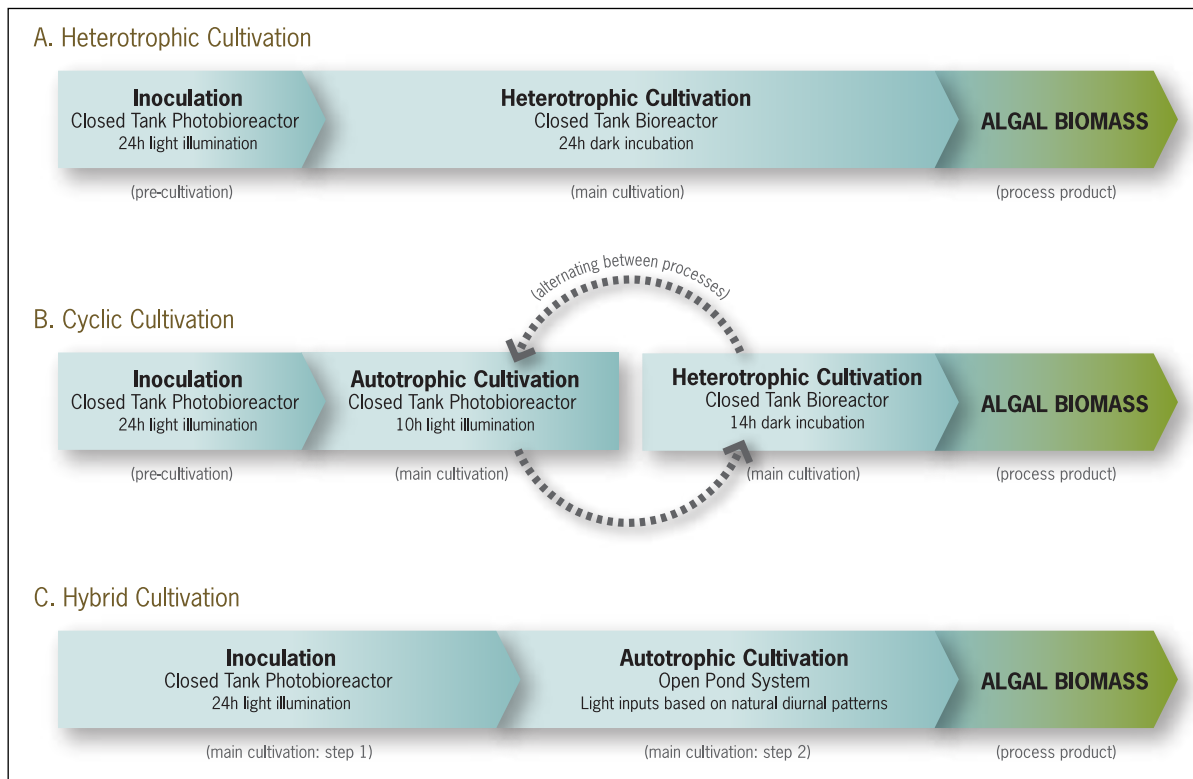
Figure 14: Cyclic cultivation combines technologies of both heterotrophic systems (A) and closed photobioreactors. Cyclic cultivation differs from hybrid cultivation in that its two methods are applied in a continuously alternating loop (B), whereas the two methods in hybrid cultivation are applied contiguously (C), but not in a repeating loop.
